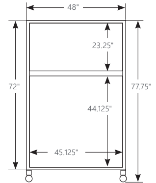
Dimensions of double sided acoustic panel with frosted acrylic top
