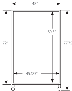
Dimensions of full size double sided acoustic panel
